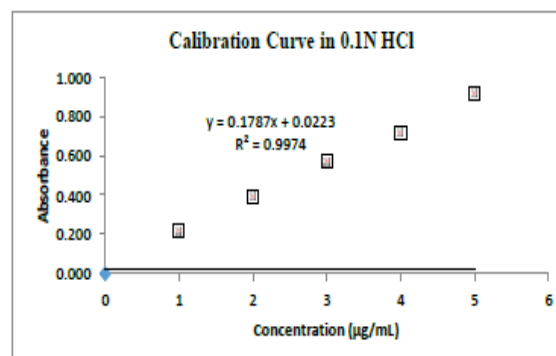
Fig: Calibration curve of Acetohydroxamic acid in 0.1N HCl (n=3)
